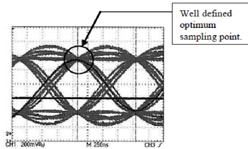
Figure 12-3. Ideal eye diagram
