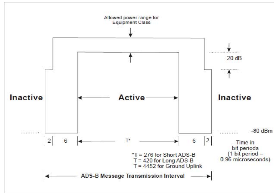
Figure 12-2. Time/amplitude profile of UAT message transmission
