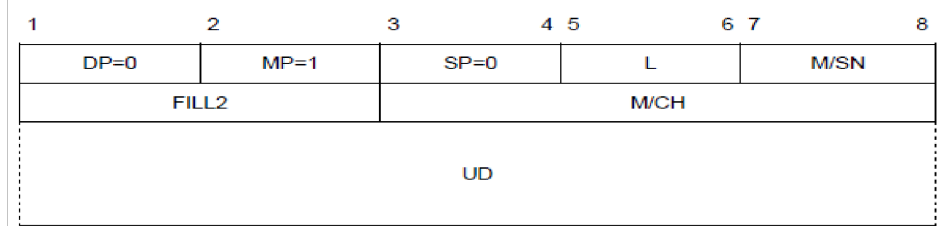
Figure 5-22. LONG FORM MSP packet
