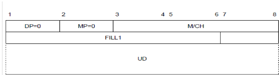
Figure 5-21. SHORT FORM MSP packet
