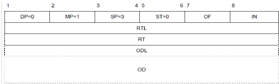
Figure 5-19. ROUTE packet
