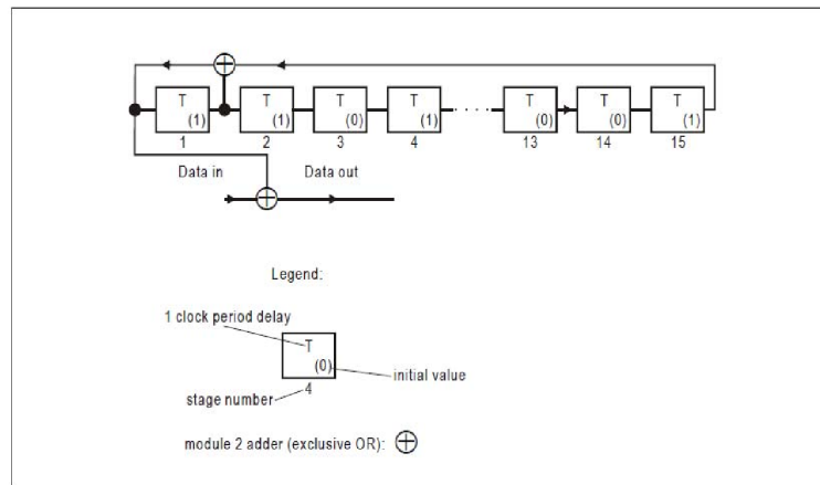
Figure 6-2. PN-generator for bit scrambling sequence
