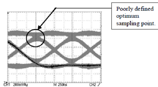
Figure 12-4. Distorted eye diagram
