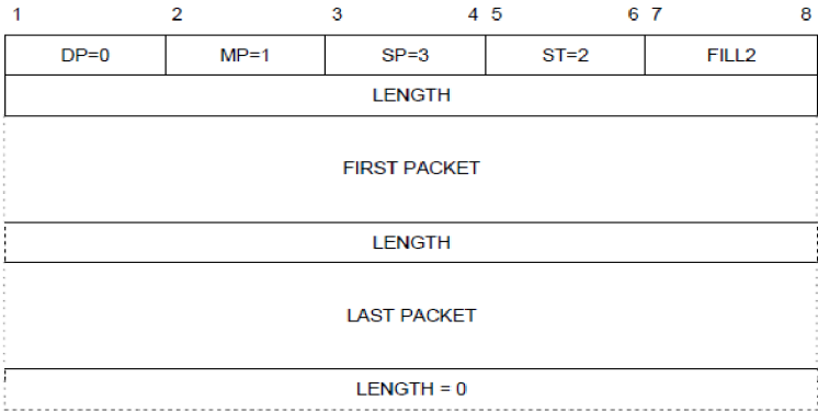
Figure 5-20. MULTIPLEX packet
