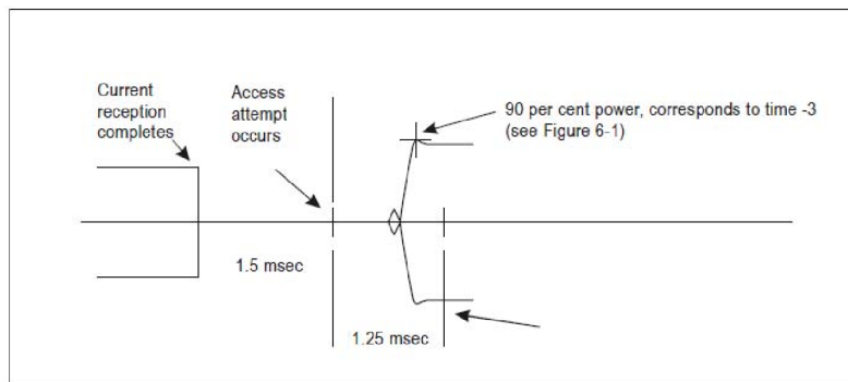
Figure 6-3. Receive to Transmit turnaround time
